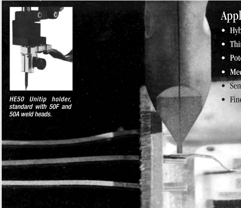
Unitip electrode bonding gold ribbon to hybrid interconnect pin.
