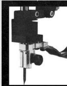
HE50 Unitip holder, standard with 50F and 50A weld heads.
