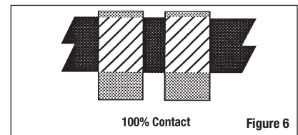
Figure 6 shows the same electrode tip offset slightly on the part, but still contacting 100% of the part width. Both figures 5 and 6 produce equal quality welds.
