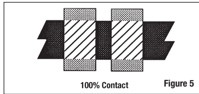
Figure 5 shows a large Unitip electrode tip centered over and completely covering 100% of the part width.
